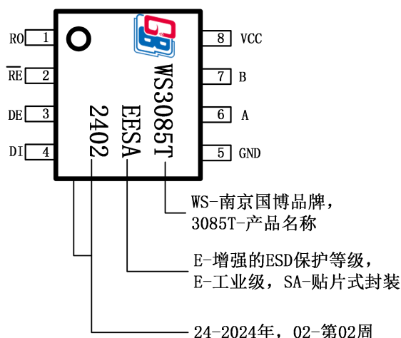
WS3085T 引脚图—8-pin SOP (Top View)
